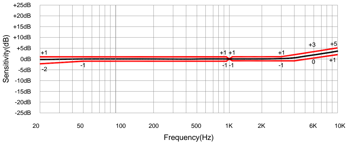
Frequency Response (0dB=1V/Pa)
