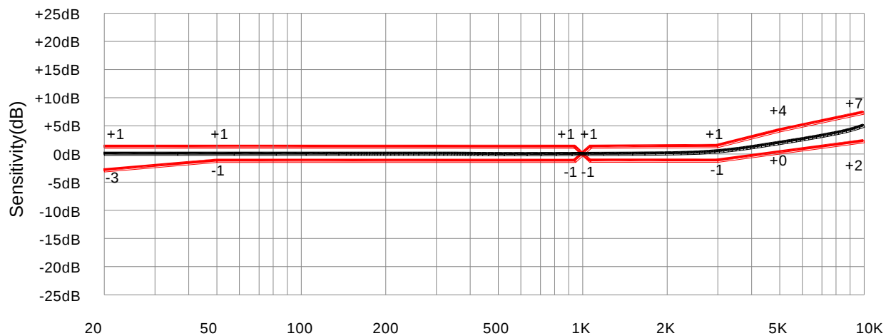
Frequency Response (0dB=1V/Pa)
